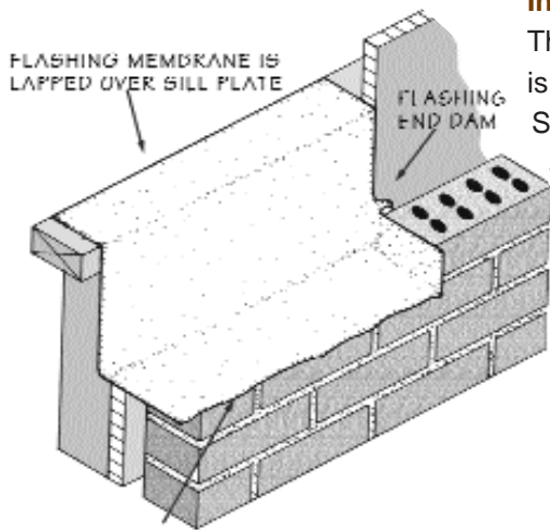
FLASHING MEMBRANE IS LAPPED OVER SILL PLATE FLASHING END DAM
